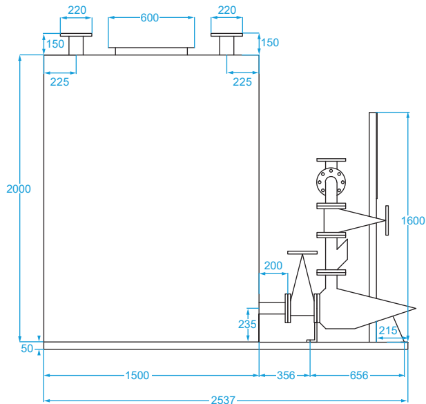
SIDE ELEVATION
