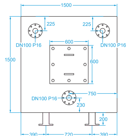
TOP OF CHAMBER
