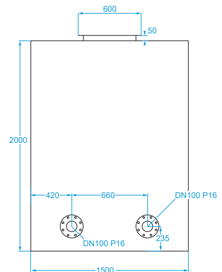
FRONT OF CHAMBER
