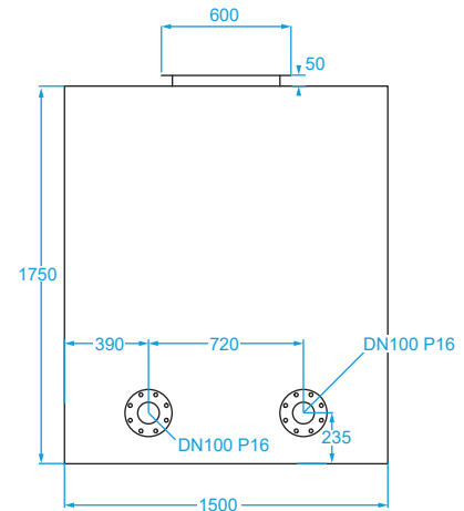
FRONT OF CHAMBER
