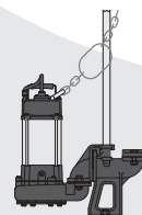
1 pedestal-mounted manual pump with guide rails and lifting chain
