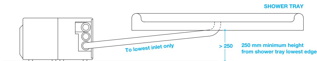
Minimum height of shower tray
