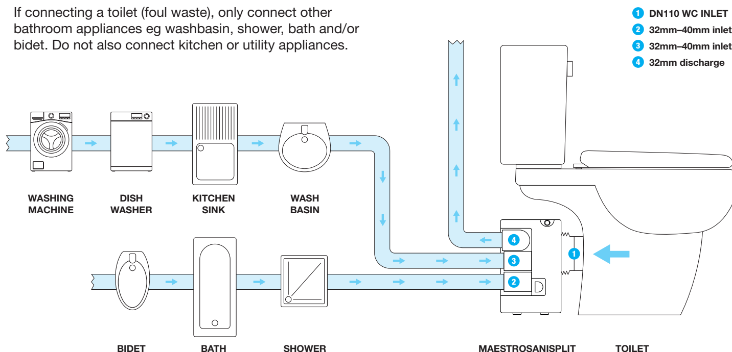
Connecting appliances to the unit
